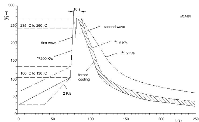
Fig. 8 Recommended wave soldering profile
